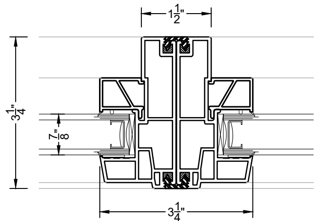
⑤ 0 DEGREE MULLION PW 211
