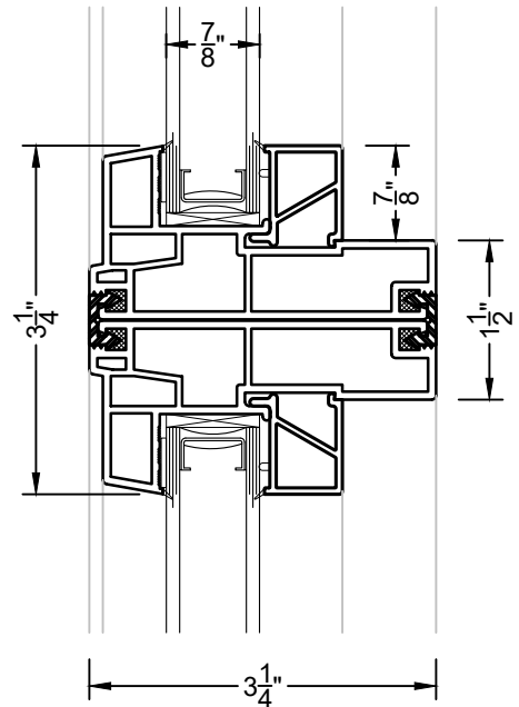
④ 0 DEGREE MULLION PW 211
