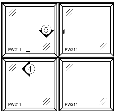
211 PICTURE WINDOW W/ 0° MULLION
