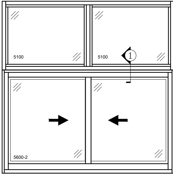
PW5100-2H OVER SL5600-2
