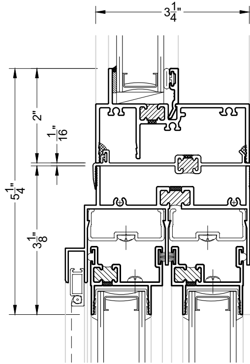
① STACK MULLION PW5100 OVER SL5600-2
