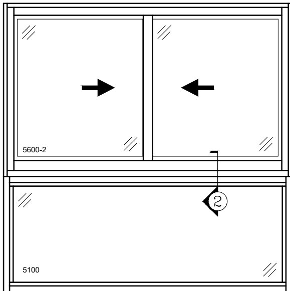
SL5600-2 OVER PW5100
