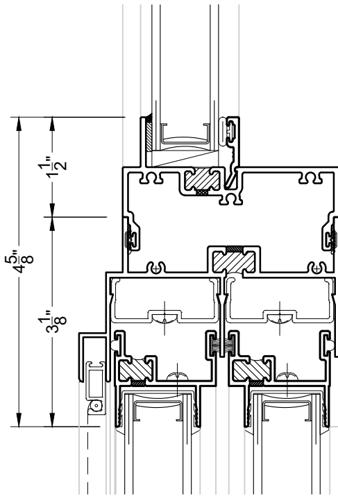
⑤ MALE FRAME MULLION PW5100 MALE OVER SL5600
