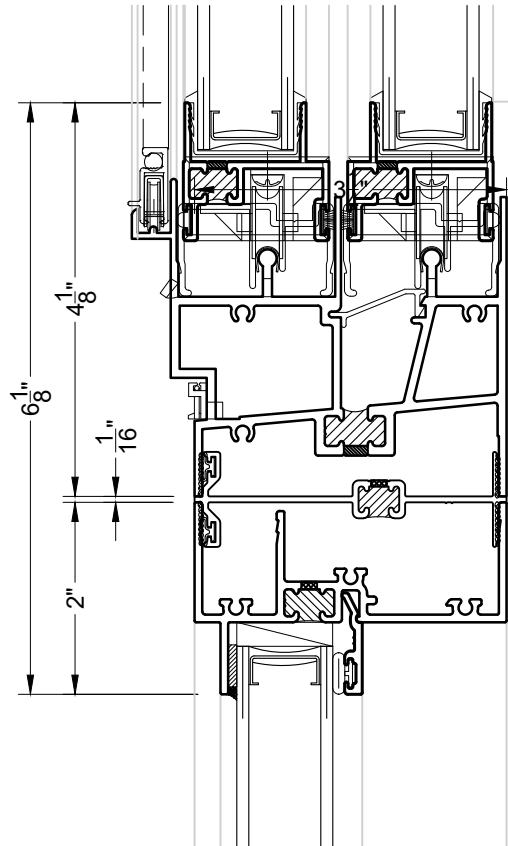
② SHORT LEG H MULLION SL5600-2 OVER PW5100
