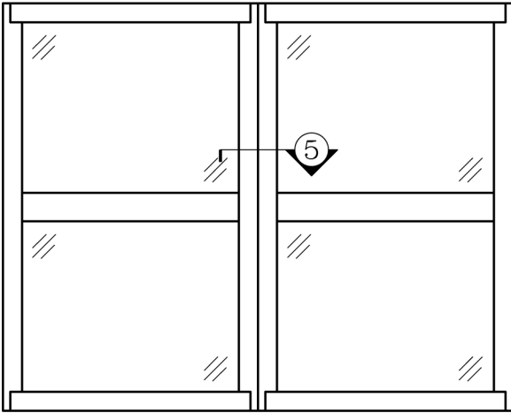
PW8510-2V & PW8510-2V WITH H MULLION
