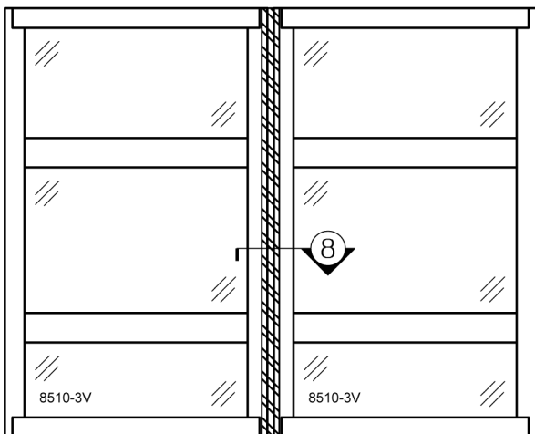
PW8510-3V & PW8510-3V WITH 3PC MULLION
