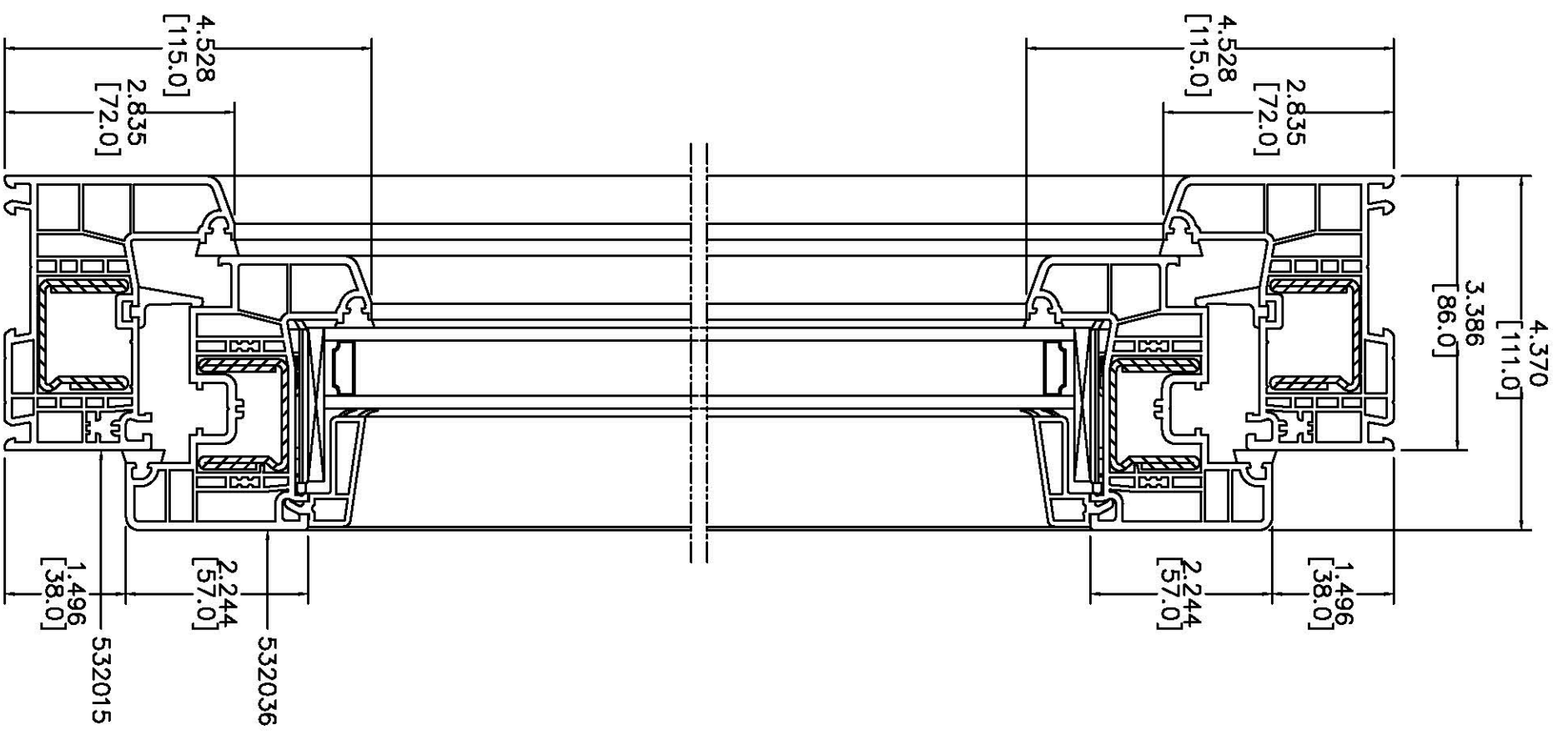
Section: A-A
