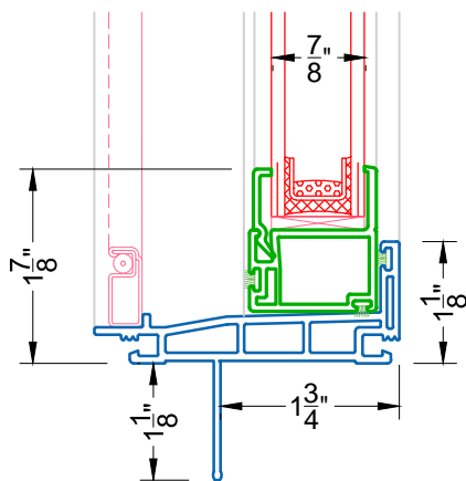
2 STANDARD SILL 340 HOPPER DOWN
