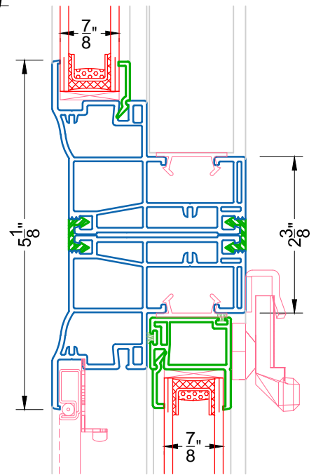
6 0 DEGREE MULLION PW 310 OVER HP 340
