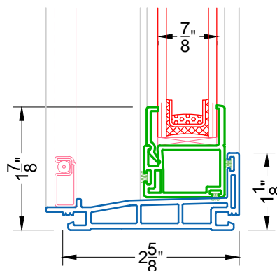
2A SILL W/O NAILING FIN 340 HOPPER DOWN FOR REPLACEMENT CONSTRUCTION OR MULLED UNIT
