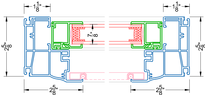
3A JAMB W/O NAILING FIN 340 HOPPER DOWN FOR REPLACEMENT CONSTRUCTION OR MULLED UNIT
