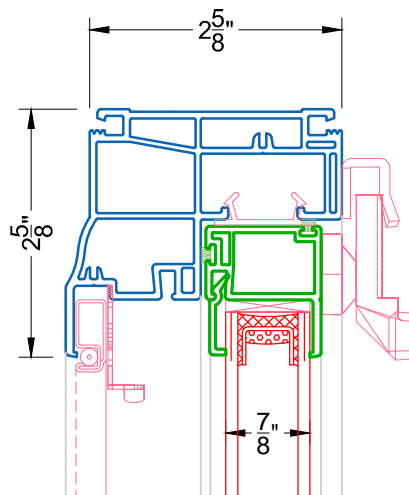
1A HEAD W/O NAILING FIN 340 HOPPER DOWN FOR REPLACEMENT CONSTRUCTION OR MULLED UNIT
