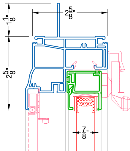
1 STANDARD HEAD 340 HOPPER DOWN
