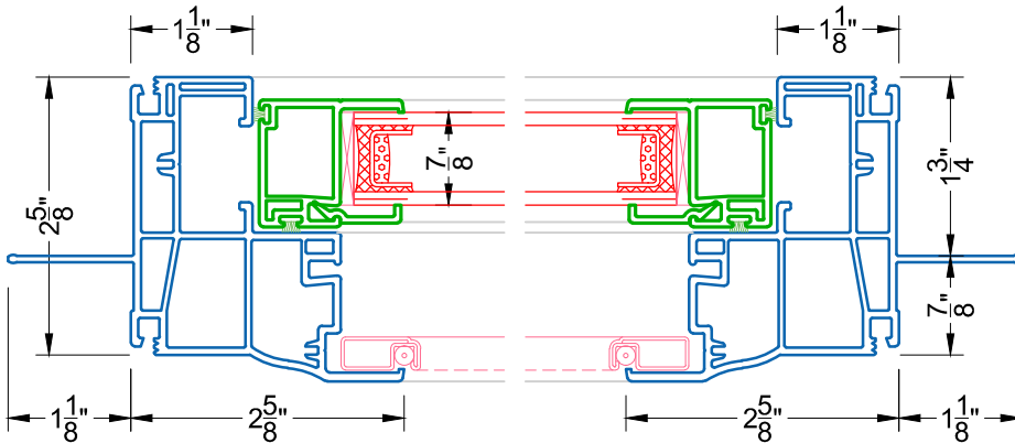
3 STANDARD JAMB 340 HOPPER DOWN
