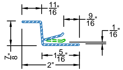
CAULK ADAPTOR A54-X010 For Frame Thickness of 1/16"
