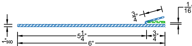
6" FRAME EXPANDER A54-X009 For Frame Thickness of 1/16"
