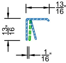
13/16" CAULK EXPANDER A54-X004 For Frame Thickness of 1/16"
