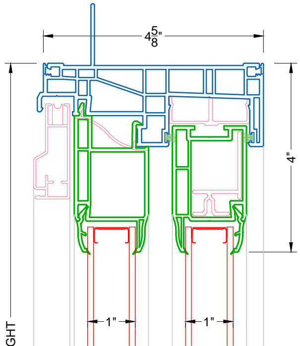
1 STANDARD HEAD 1500 SLIDING DOOR
