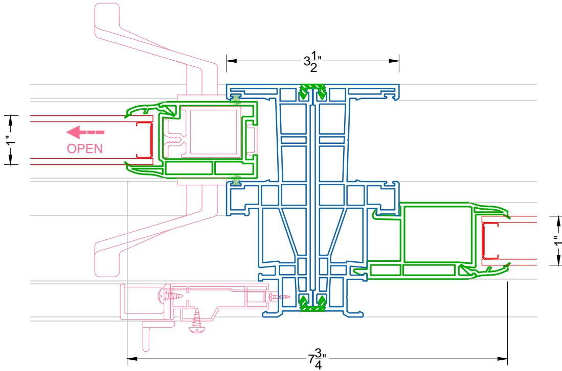
8 0 DEGREE MULLION 1500 SLIDING DOOR & SIDE LITE
