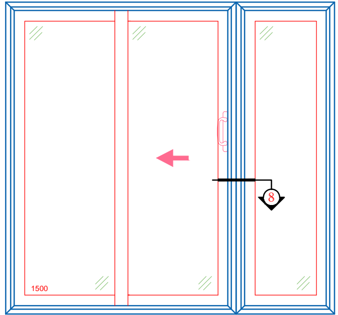
1500 O-X SLIDING DOOR WITH SIDE LITE
