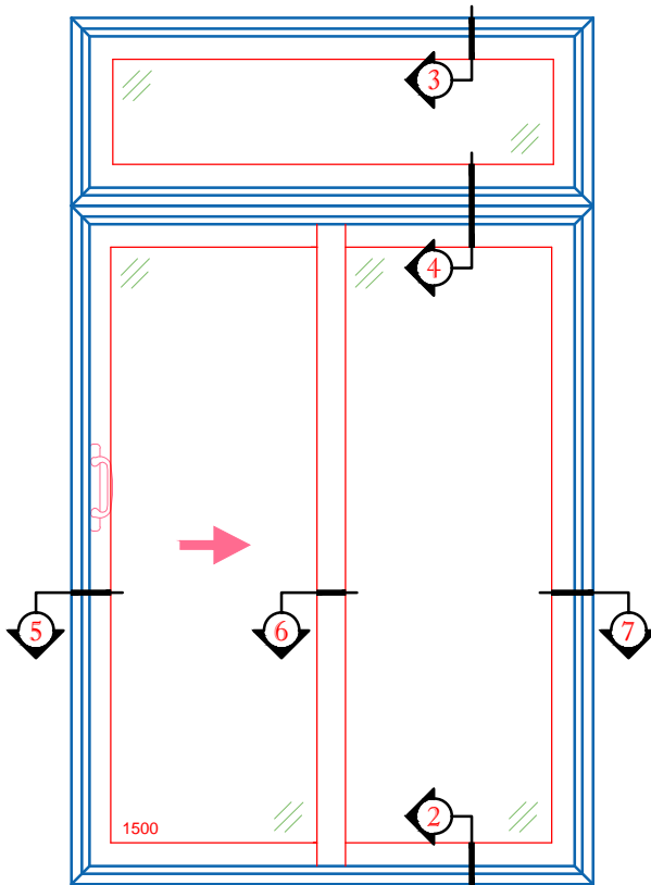
1500 X-O SLIDING DOOR W/ TRANSOM
