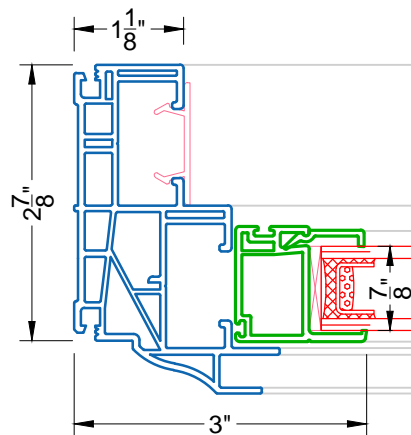
①A FRAME W/O NAILING FIN PW 410 FOR REPLACEMENT CONSTRUCTION OR MULLED UNIT
