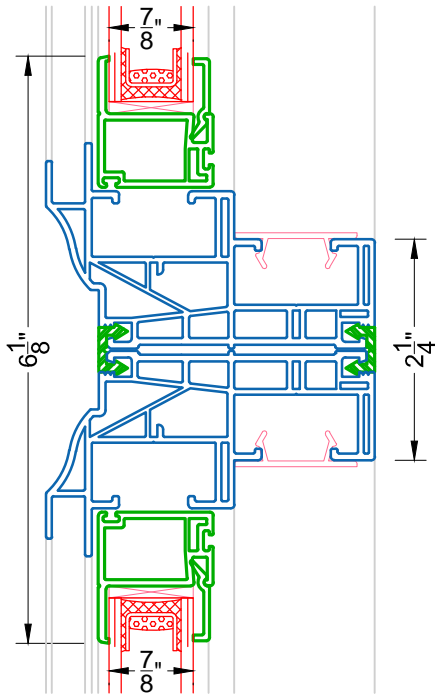
5 0 DEGREE MULLION PW 410
