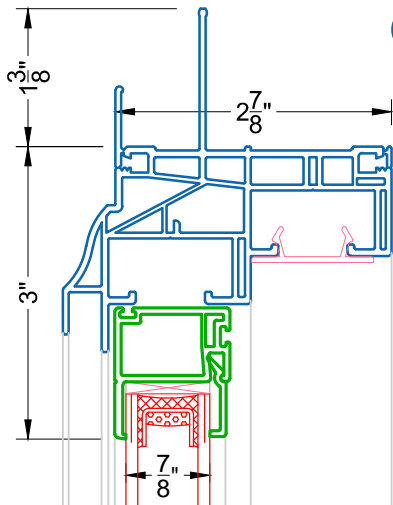
③ STANDARD HEAD PW 410
