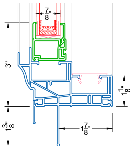
④ STANDARD SILL PW 410
