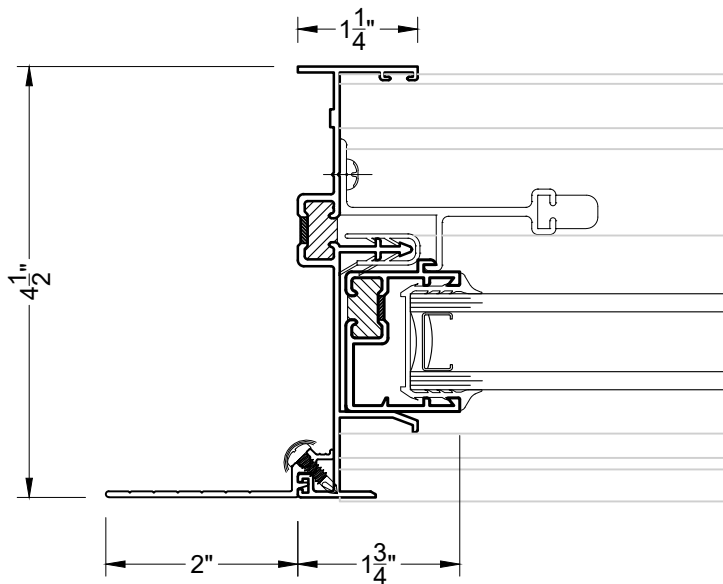
④ 2" SCREW ON FLANGE JAMB 1240
