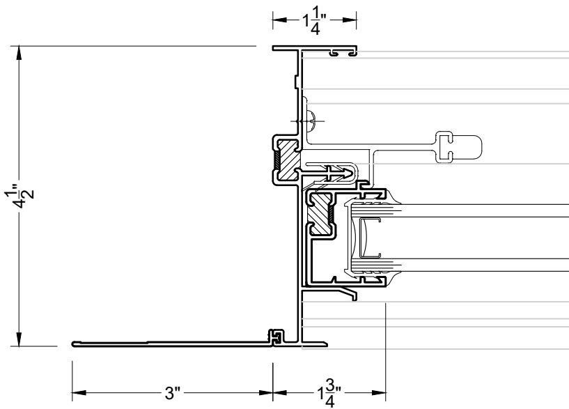
④A JAMB W/ 3" SLIDE ON FLANGE 1240
