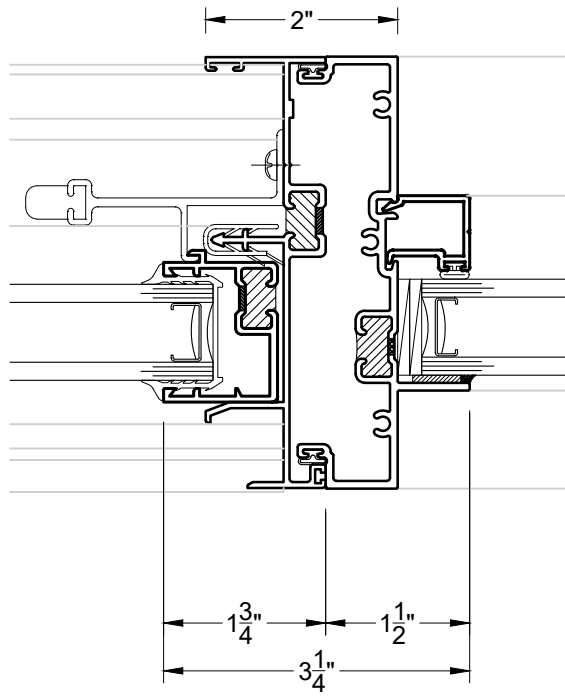
8A MALE FRAME MULLION 1240 W/ 1270A SIDELITE
