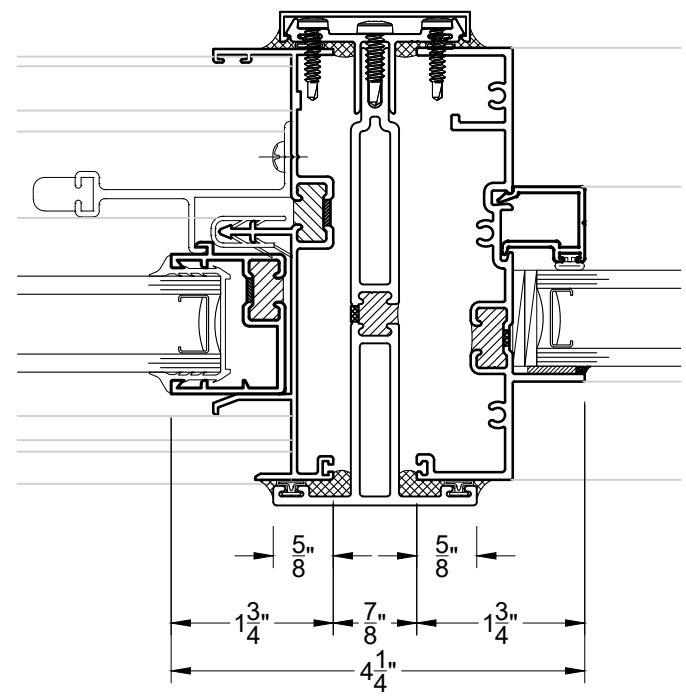
8B 3PC MULLION 1240 W/ 1270A SIDELITE
