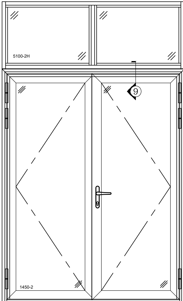
PW5100-2H TRANSOM OVER CTT1450-2 W/ H MULLION
