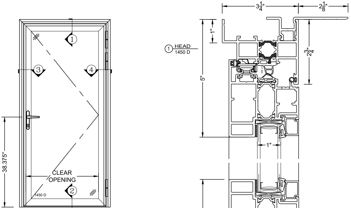
1450 OUT-SWING ADA THRESHOLD
