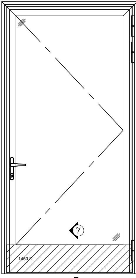
1450 OUT-SWING ADA THRESHOLD WITH 10" KICK PLATE
