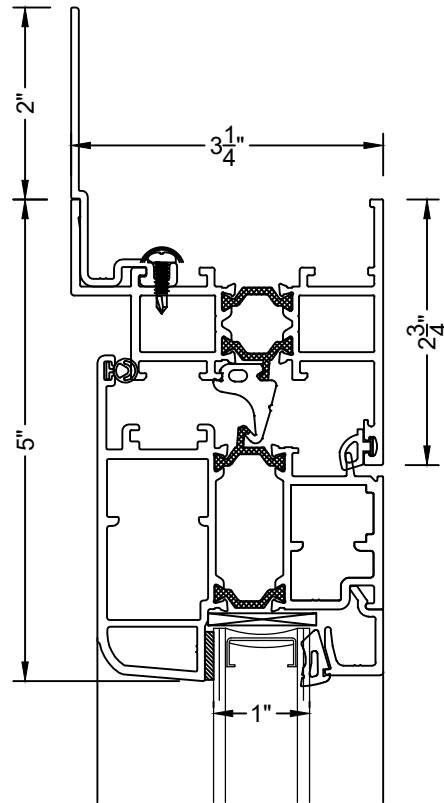
①A 2" APPLIED ON FLANGE HEAD CTT1450
