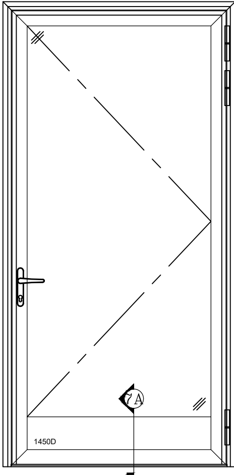
1450 OUT-SWING ADA THRESHOLD WITH EXTRUDED KICK PLATE
