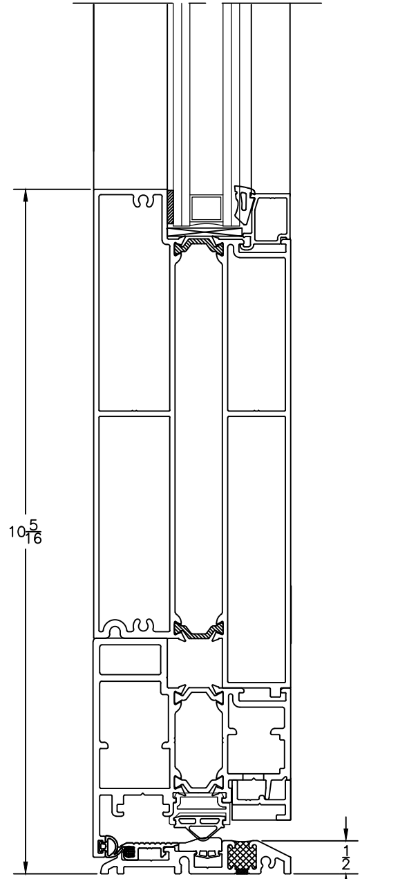
7A ADA SILL W/ EXTRUDED KICK PLATE 1450 OUT-SWING DOOR
