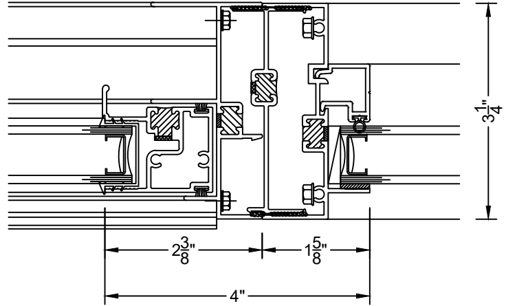
⑨ SHORT LEG H MULLION SL2300 & 2100 PW
