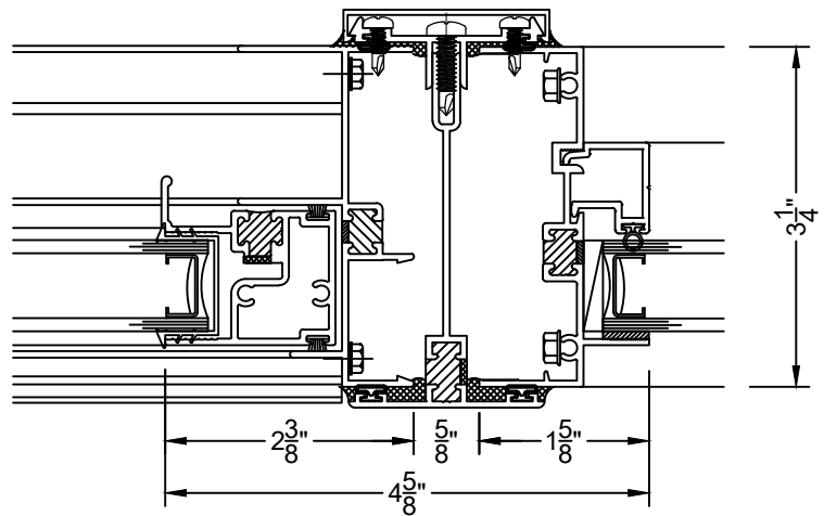
⑩ 3PC MULLION SL2300 & 2100 PW
