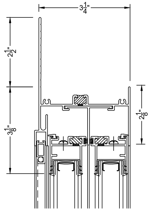
①A 2-1/2" FLANGE HEAD SL2300
