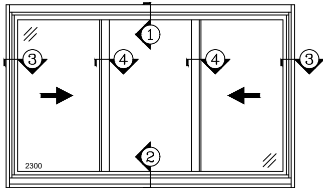
2300-3 THREE LITE SLIDER EQUAL LITE (X-O-X)
