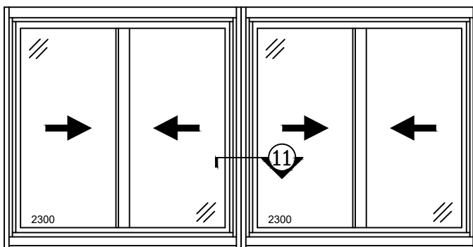
SL2300-2 & SL2300-2 W/ 2000A H-MULLION
