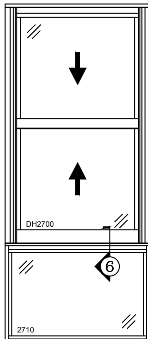
DH2700 OVER 2710
