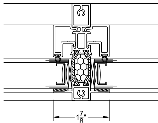
⑧ T MULLION 2710 & 2710
