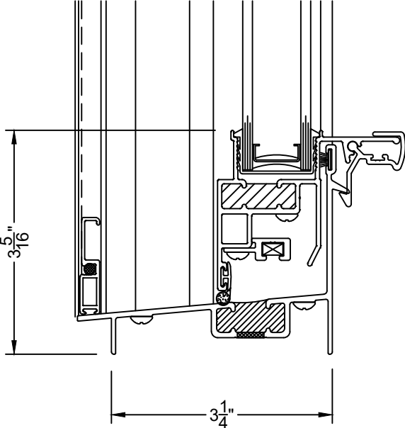
③ SILL DH2700
