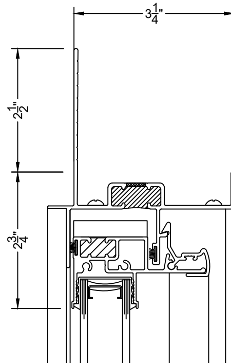
①B 2.5" FLANGE HEAD DH2700
