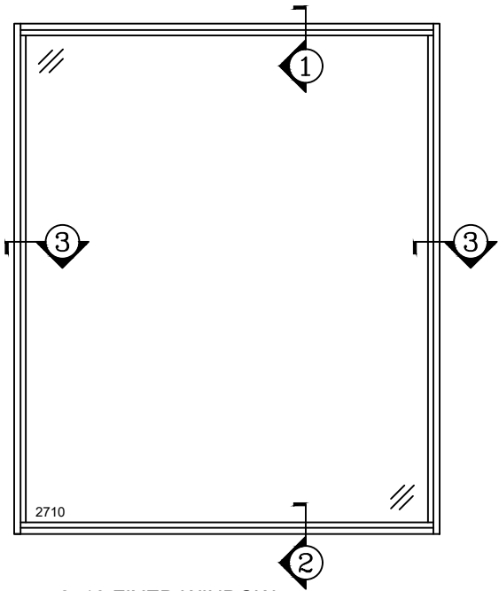
2710 FIXED WINDOW
