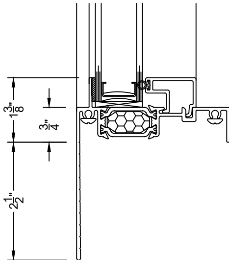
②C 2.5 FLANGE SILL 2710
