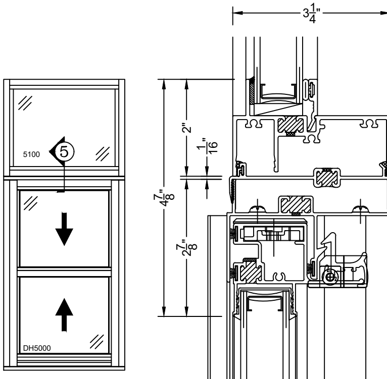
PW5100 OVER DH5000
