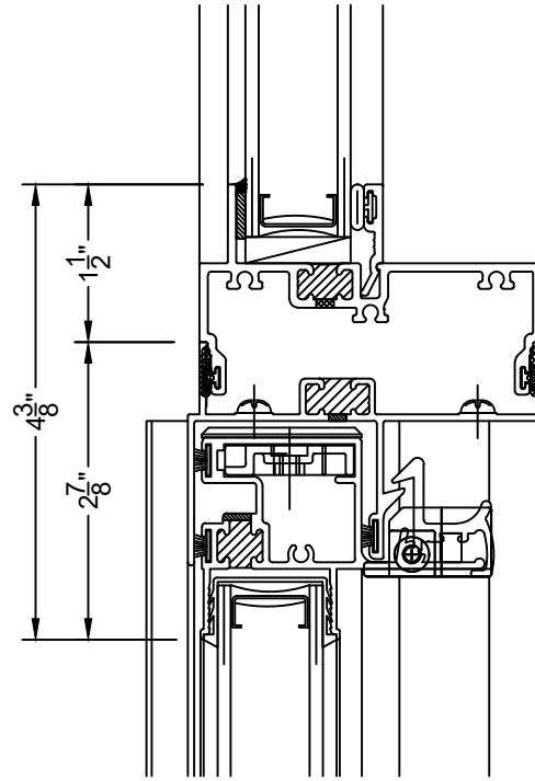
5B MALE FRAME MULLION PW5100 MALE OVER DH5000
