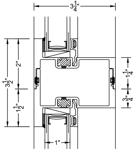
⑩ HEAVY DUTY MALE / FEMALE FRAME PW5100
