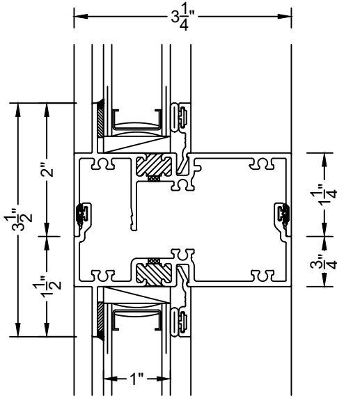
⑨ MALE / FEMALE FRAME PW5100
