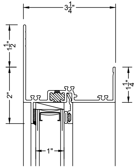
①A 1-1/2" FLANGE HEAD/SILL PW5100
