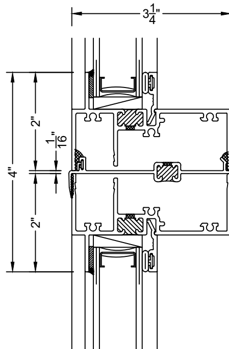
⑤ STACK MULLION PW5100 OVER PW5100
