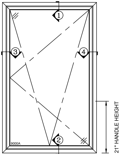
9000A TILT & TURN WINDOW
