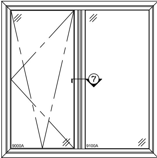
9000A-2H TILT & TURN & FIXED
