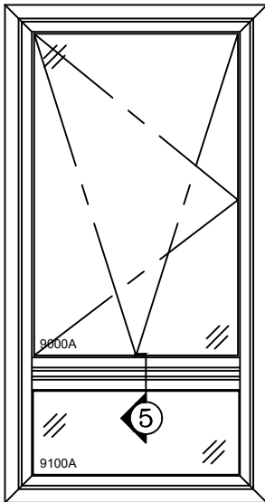
9000A-2V TILT & TURN OVER FIXED
