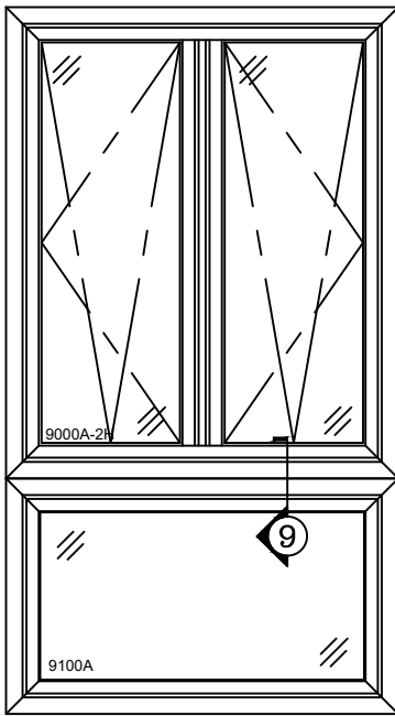
9000A-2H TWIN OVER 9100A
