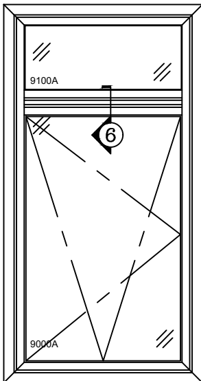
9000A-2V FIXED OVER TILT & TURN
