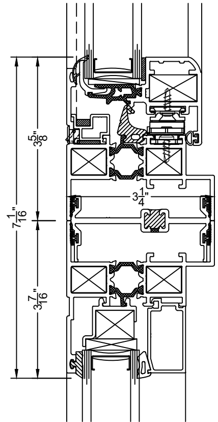
9A H MULLION 9000A OVER 9100A
