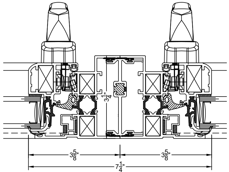
10 H MULLION 9000A & 9000A
