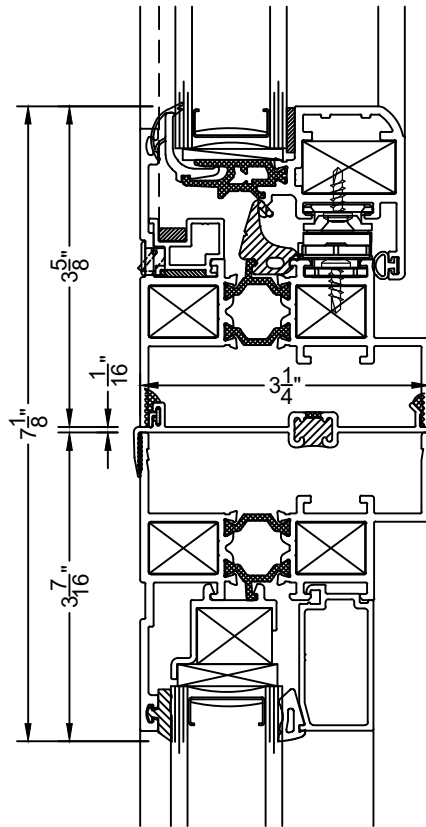
9 STACK MULLION 9000A OVER 9100A
