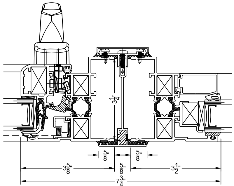
11 3PC MULLION 9000A & 9100A
