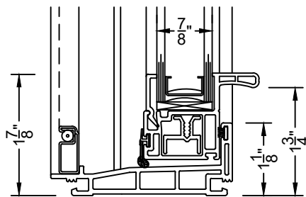
② REPLACEMENT SILL SH300R
