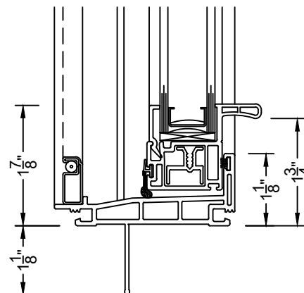
③ SILL SH300
