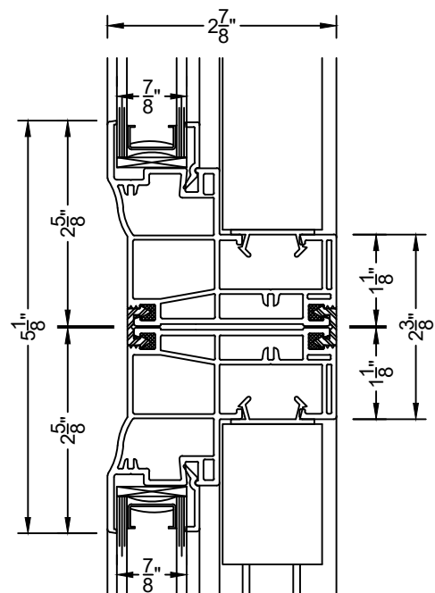
④ 0 DEGREE MULLION PW310 OVER SH300
