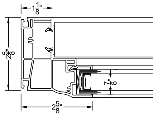
③A FRAME W/O NAILING FIN PW 310
