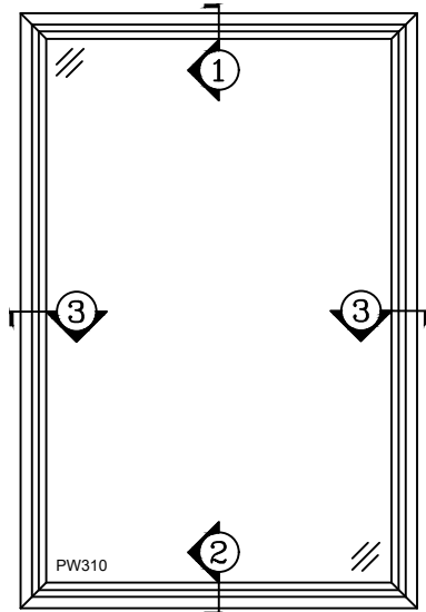
310 PICTURE WINDOW
