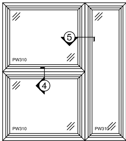
310 PICTURE WINDOW W/ 0° MULLION & H-MULLION
