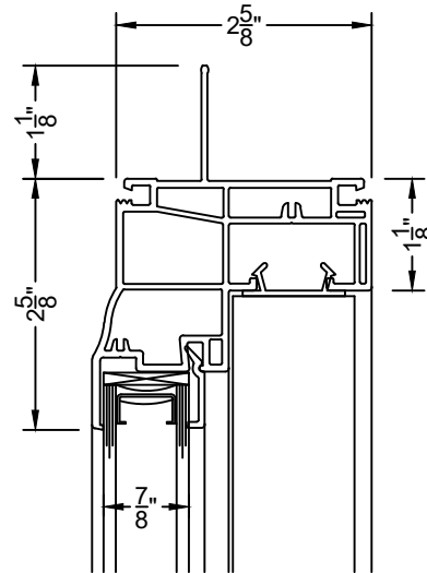
① HEAD PW310
