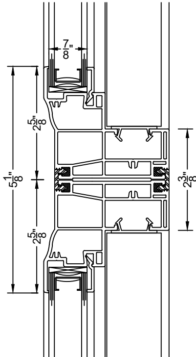
④ 0 DEGREE MULLION PW 310
