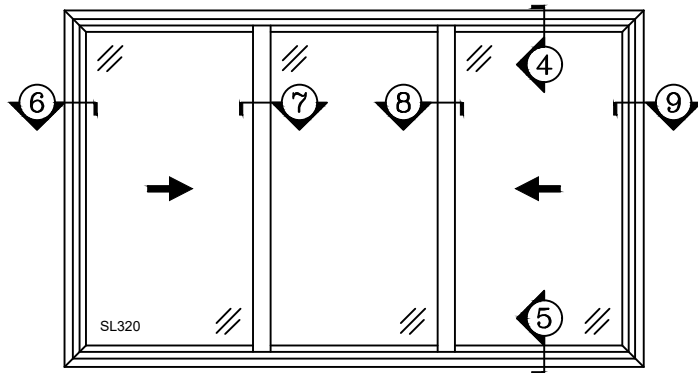
320-3 THREE-LITE SLIDER X-O-X (EQUAL 1/3, 1/3, 1/3)
