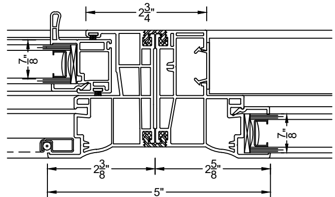
⑩ 0 DEGREE MULLION SL320 & PW310
