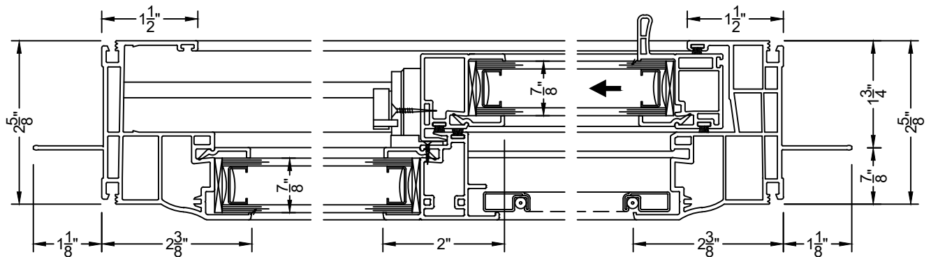
① JAMB AT FIXED SIDE SL320
