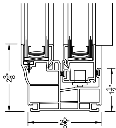
⑤A SILL W/O NAILING FIN SL320
