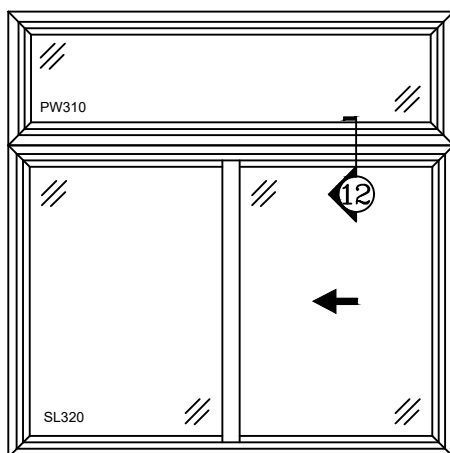
PW310 OVER 320-3 THREE-LITE SLIDER
