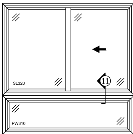
320-2 TWO-LITE SLIDER OVER PW310
