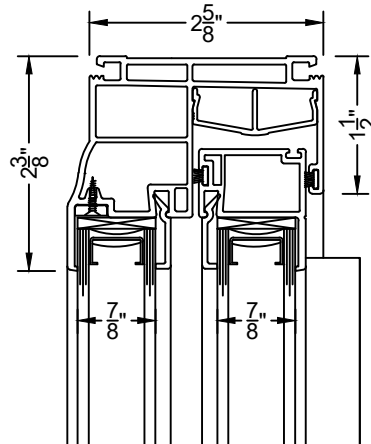
④A HEAD W/O NAILING FIN SL320
