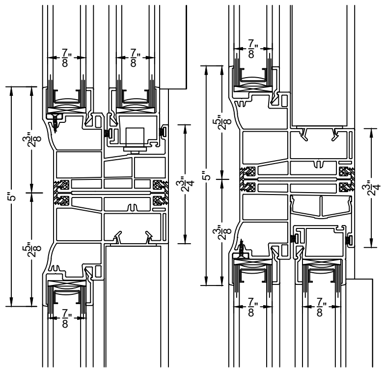
⑪ 0 DEGREE MULLION SL320 OVER PW310
