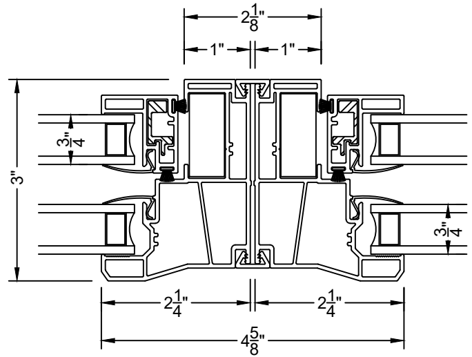
(7) MULLION (0 DEGREE) SH800-SH800
