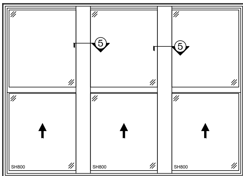
TRIPLE SH800
