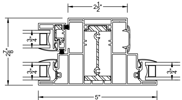
⑥ INTERMEDIATE JAMB SH800/PW810
