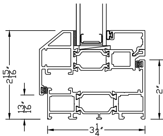
STANDARD EQUAL LEG FRAME
