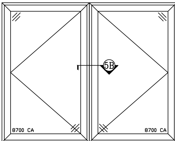
8700 TWIN CASEMENT (FIELD MULLED W/ INTERIOR MULL)
