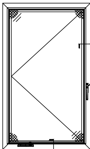
INTERIOR VIEW 8700 OUT-SWING CASEMENT WITH OPERATOR
