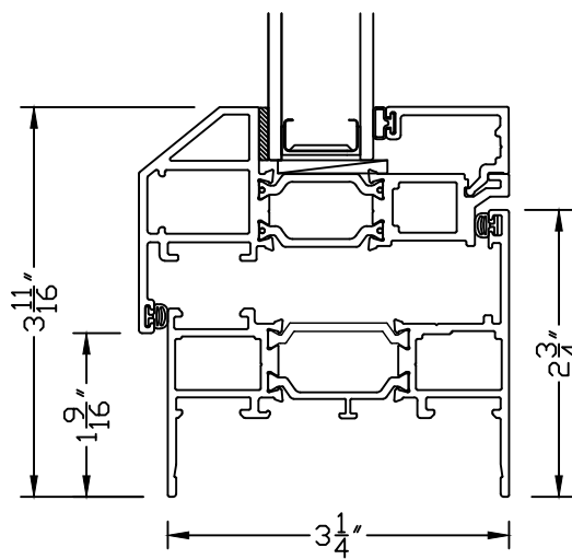
FRAME W/ LEG EXTENSION
