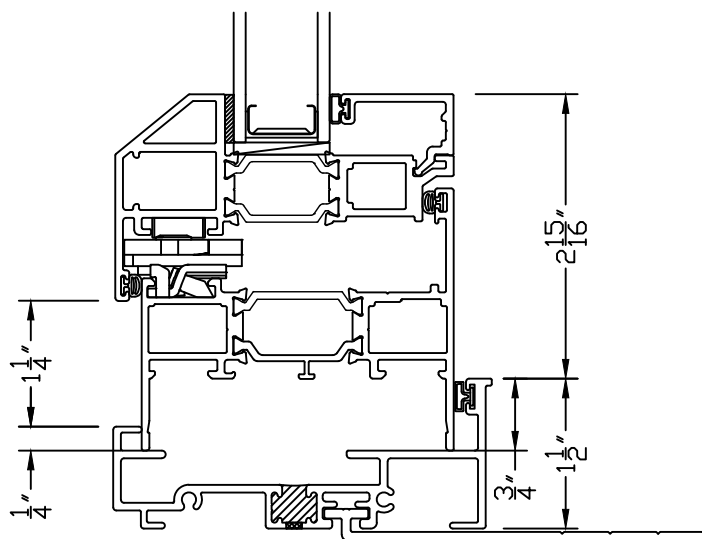
①⑧ 3/4" FRAME EXTENSION @ SILL 8700 CA
