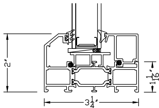
STANDARD BEVELED EQUAL LEG FIXED FRAME
