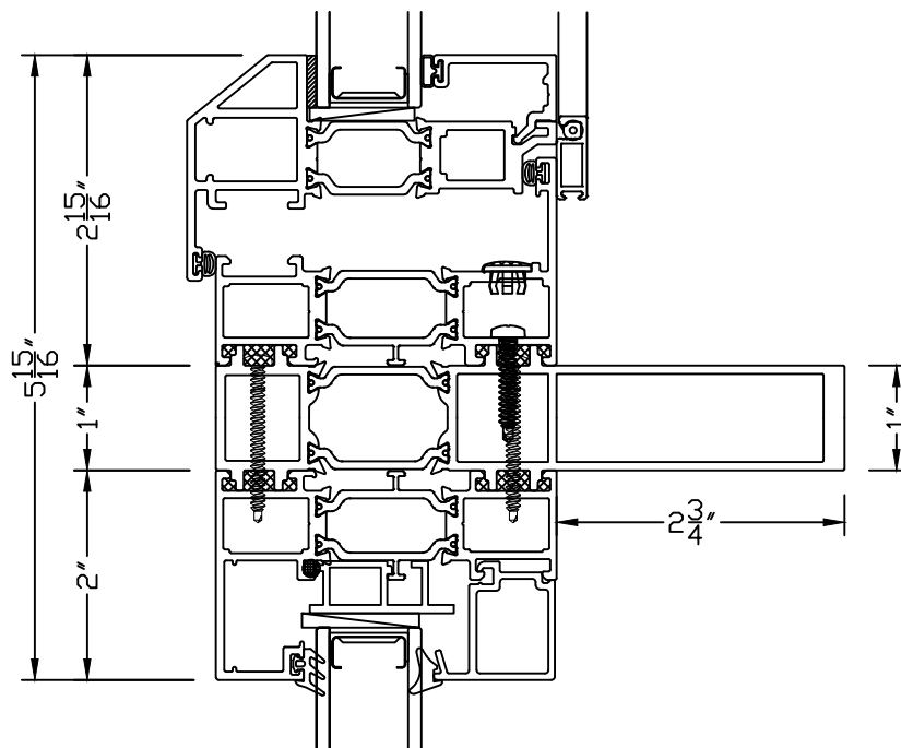
15B EXTENDED STRUCTURAL MULLION 8700 CA OVER FX
