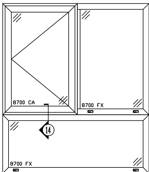
8700 CA OVER FX (FIELD MULLED W/ INTERIOR MULLION)
