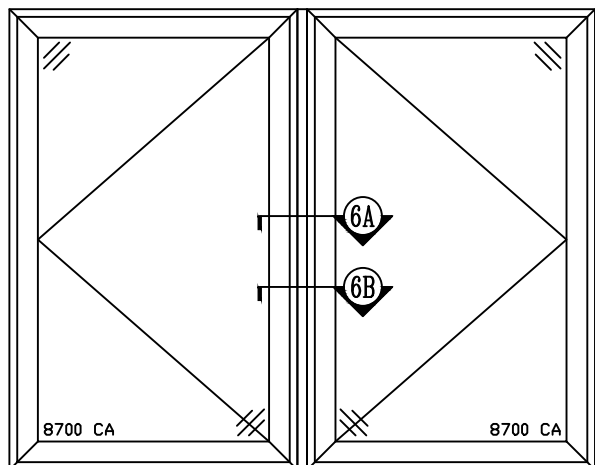
8700 TWIN CASEMENT (FIELD MULLED W/ STRUCTURAL MULLION)
