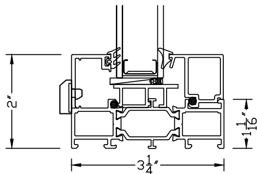
STANDARD EQUAL LEG FIXED FRAME
