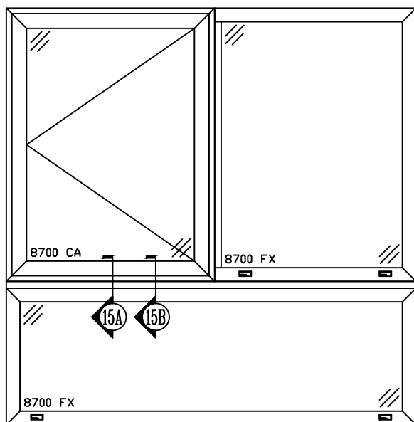
8700 CA OVER FX (FIELD MULLED W/ STRUCTURAL MULLION)
