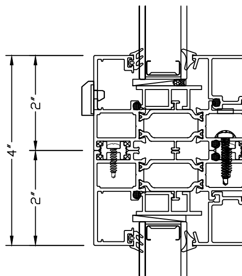
⑪ INTERIOR MULLION 8700 FX OVER FX
