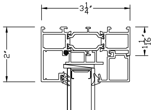
① HEAD 8700 FX
