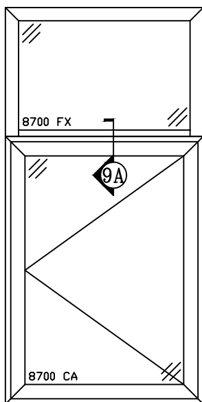
8700 FX OVER CA (W/ MASTERFRAME)
