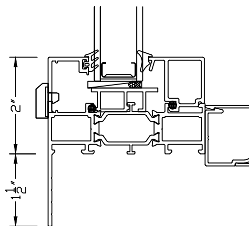
①⑨ SILL W/ FACE FLANGE 8700 FX
