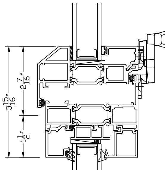
9B C MULLION 8700 PD OVER FX
