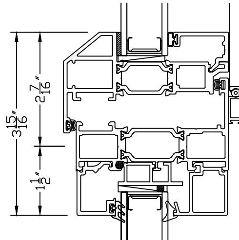
⑬ C MULLION 8700 CA OVER FX
