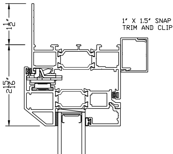
①⑦ HEAD W/ FACE FLANGE 8700 CA
