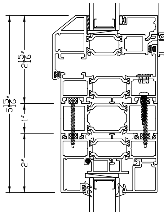
15A STRUCTURAL MULLION 8700 CA OVER FX
