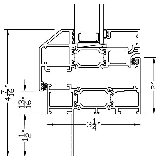
FRAME W/ 1.5 NAILING FIN
