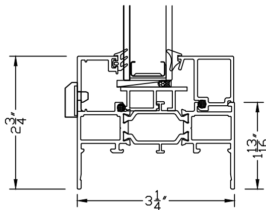
FIXED FRAME W/ LEG EXTENSION
