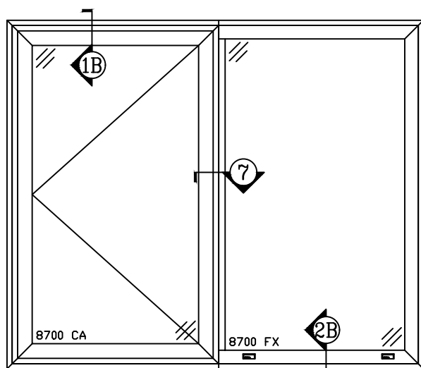
8700 CA & FX WITH C MULLION (MASTERFRAME W/ FRAME EXTENSION)
