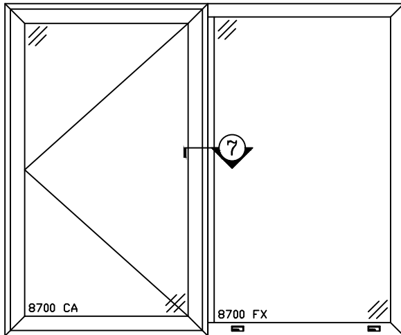
8700 CA & FX WITH C MULLION (MASTERFRAME)
