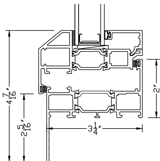
FRAME W/ 1.5 EXTERIOR FLANGE
