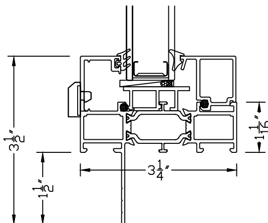
FIXED FRAME W/ 1.5 NAILING FIN
