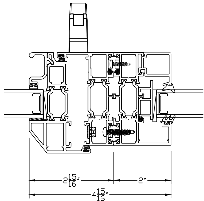
⑧ INTERIOR MULLION 8700 CA & FX
