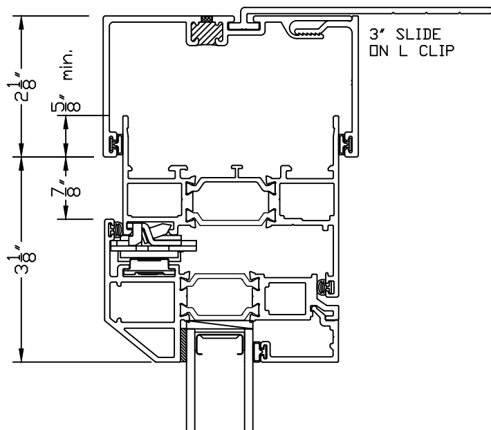
①⑥ 3/4" FRAME EXTENSION @ HEAD 8700 CA
