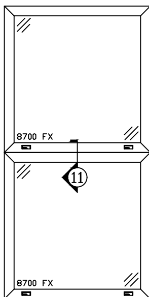
8700 FX OVER FX (FIELD MULLED W/ INTERIOR MULL)
