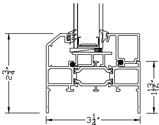
BEVELED FIXED FRAME W/ LEG EXTENSION
