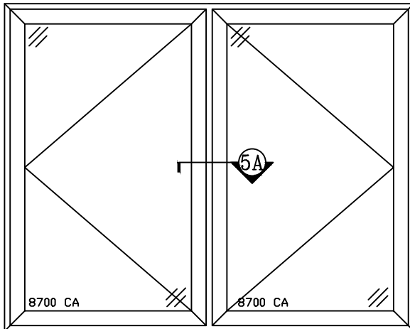
8700 TWIN CASEMENT (MASTERFRAME CONTINUOUS HEAD AND SILL W/ IMPOST)
