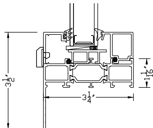
FIXED FRAME W/ 1.5 EXTERIOR FLANGE
