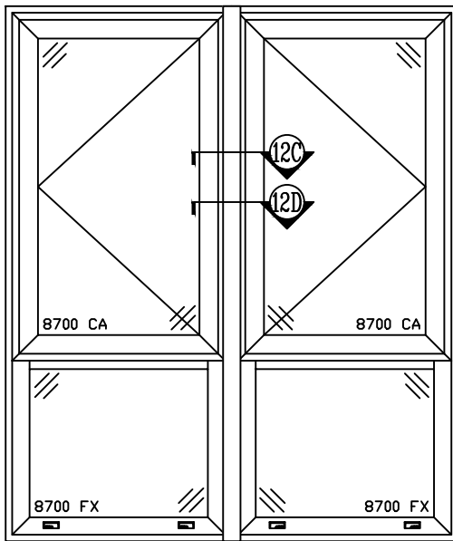
8700 CA OVER FX (FIELD MULLED W/ 3-PC MULLION & LEG EXTENSION)
